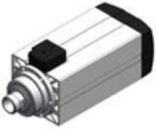
MT1120 - Y616112017 Kw 13,50 S1/16,20-S6 - connection ER40 collet - 12.000rpm - rated voltage 380V - right rotation
